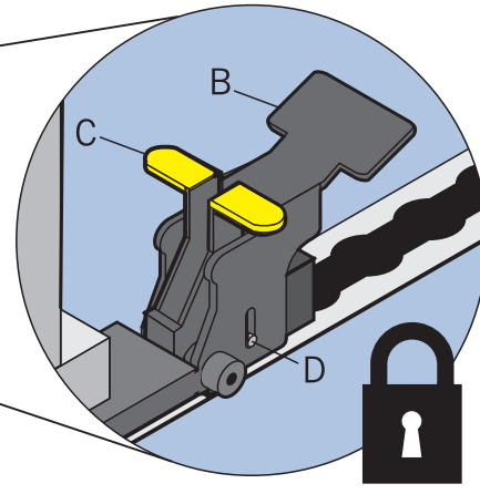
If the fitting is not in the correct position the pedal clamp B will not clamp and the safety lock C will not be in the lowered position
